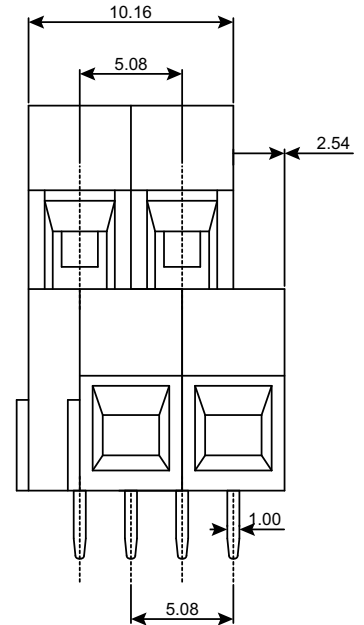
58DDS MS (2 WAY INTERLOCKED)
